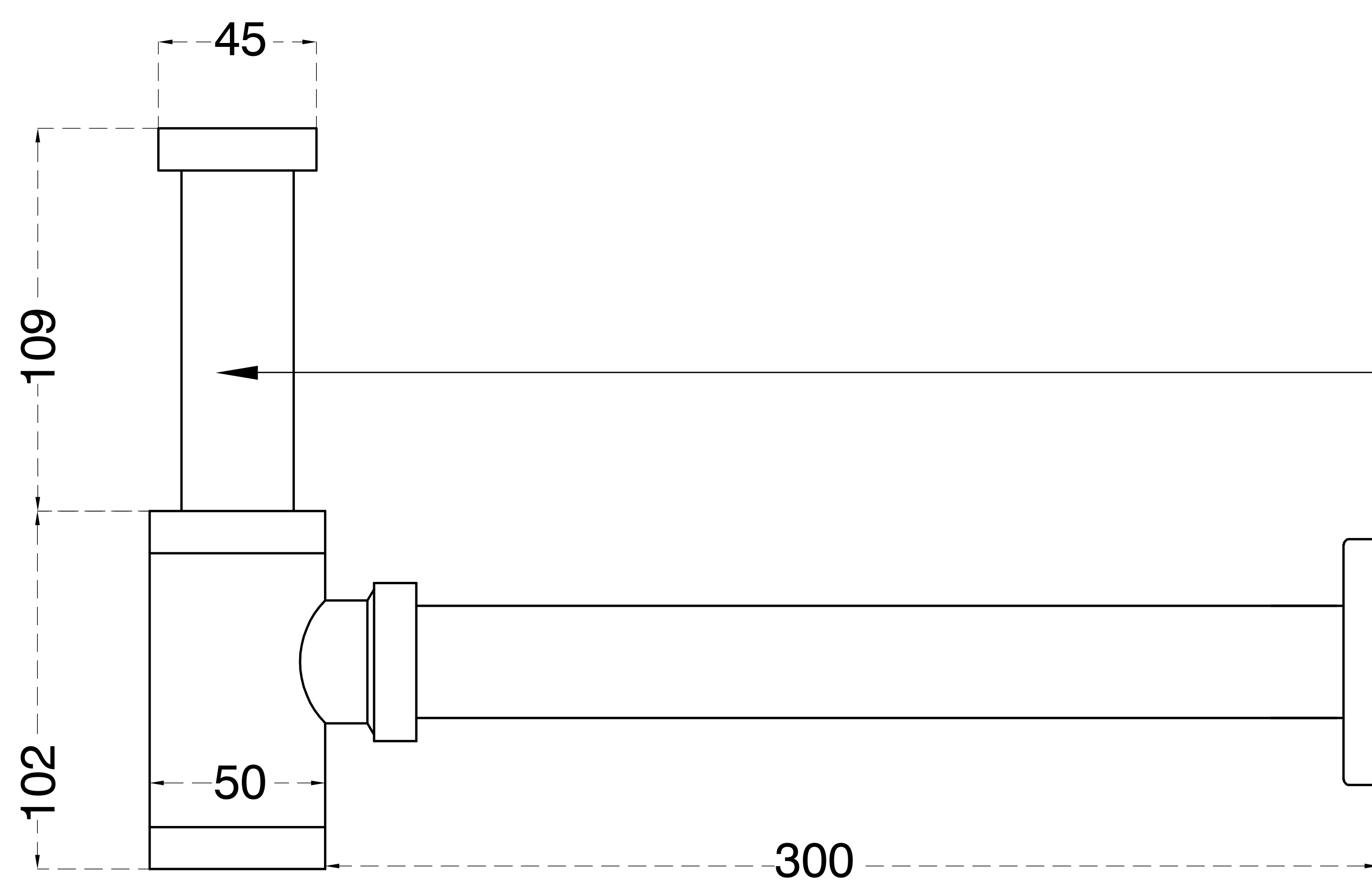
SIDE ELEVATION
